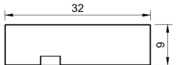
Demo valve (polycarbonate)
