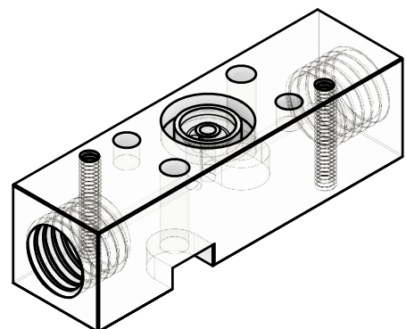
Demo valve (polycarbonate)
